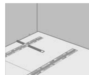
Fit the fixing strips
