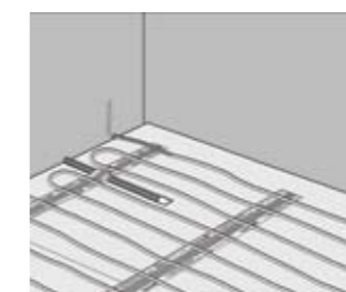
Fit the wire, replace the cover strip
